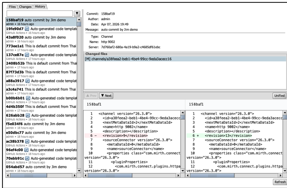
Figure 6: History tab showing commit list and diff viewer
