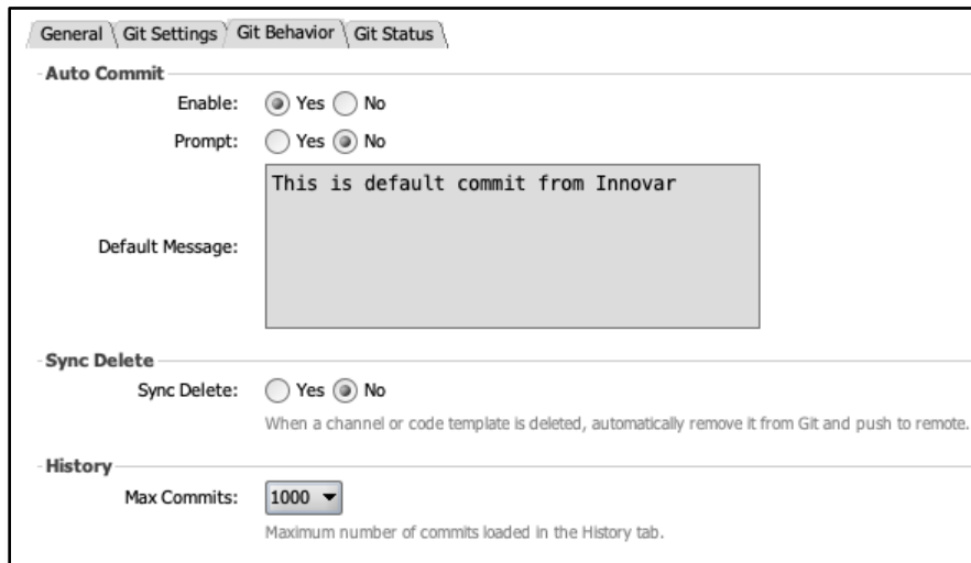
Figure 3: Git Behavior tab showing Auto Commit, Sync Delete, and History settings
