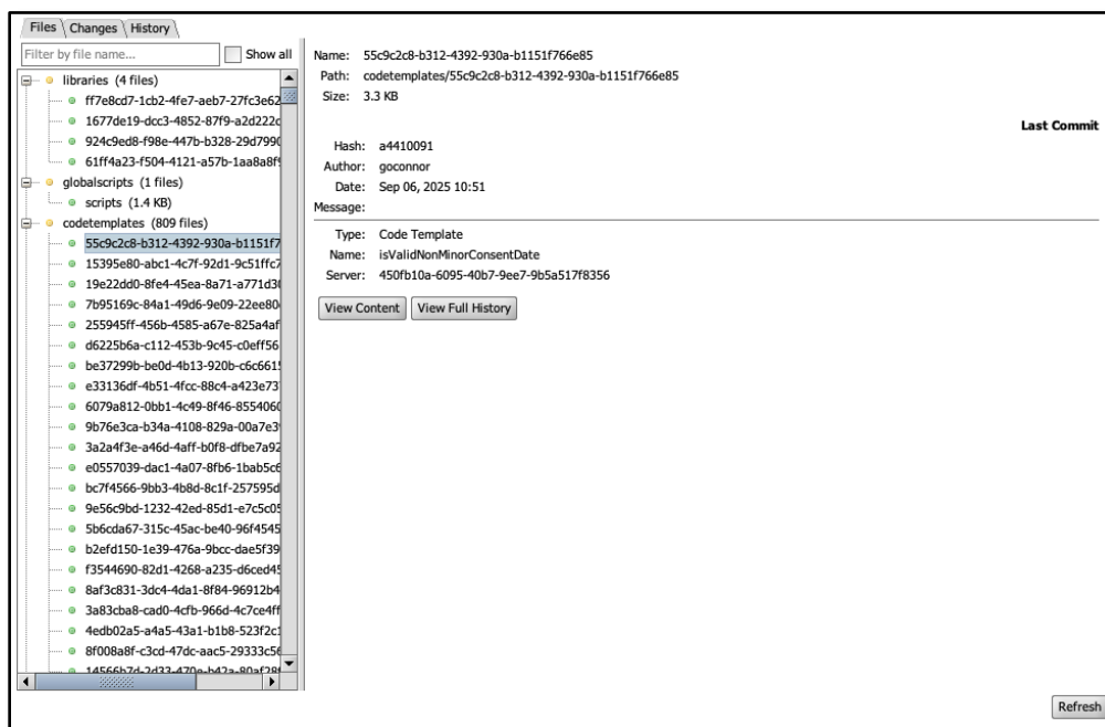
Figure 4: Files tab showing tracked files organized by category
